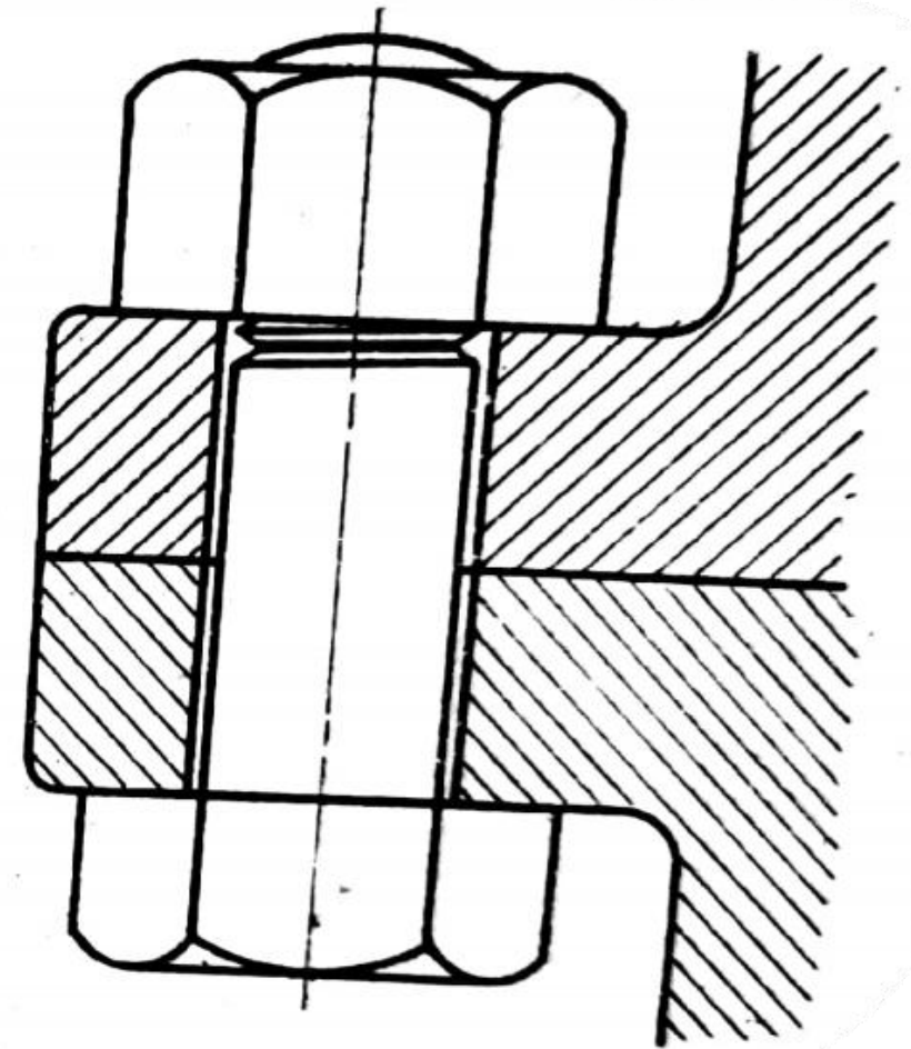
BOLTED JOINT
